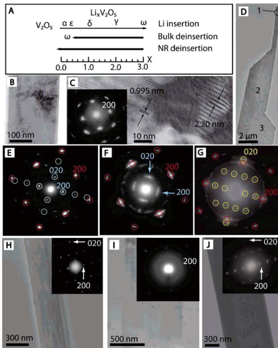
Figure 3. (A) Schematic of different \text{Li}_x\text{V}_2\text{O}_5 phases corresponding to the amount of Li inserted ( x ) per \text{V}_2\text{O}_5 unit. During Li intercalation, \text{V}_2\text{O}_5 adopts the \alpha - through \omega - \text{Li}_x\text{V}_2\text{O}_5 phases. During delithiation in the bulk, the structure remains in the \omega -phase and Li is removed to x = 0.4 . However, in our NRs, the \omega -phase is transformed back to the original pristine \text{V}_2\text{O}_5 with a full removal of Li. (B) Low-magnification TEM image of a 100 nm thick \text{Li}_x\text{V}_2\text{O}_5 NR showing contrast differences indicating structural inhomogeneity. (C) High-resolution TEM image of \text{Li}_x\text{V}_2\text{O}_5 NR with cubic SAED taken along the \langle 001 \rangle zone axis. The contrast differences and Moiré patterns with spacings of 0.995 and 2.20 nm are present. (D) 150 nm thick \text{Li}_x\text{V}_2\text{O}_5 NR with different SAED patterns at different widths along its \langle 020 \rangle direction. Location 1 corresponds to a width of 400 nm, location 2 is 2.5 \mu\text{m} , and location 3 is 3.5 \mu\text{m} . (E–G) SAED of the locations 1–3 showing different phases at different NR widths. The zone axis is the \langle 001 \rangle . The \omega - \text{Li}_3\text{V}_2\text{O}_5 cubic structure is present in all locations and is indicated by the red circles. (E) SAED at location 1. The blue circles match the \gamma - \text{Li}_2\text{V}_2\text{O}_5 orthorhombic structure. (F) SAED at location 2. The fainter, elongated spots marked with blue arrows as well as the broad ring correspond to \gamma - \text{Li}_2\text{V}_2\text{O}_5 . (G) SAED at location 3. The yellow spots correspond to pristine \text{V}_2\text{O}_5 , indicating that this region has un lithiated domains coexisting with \omega - \text{Li}_3\text{V}_2\text{O}_5 . (H) 100 nm thick and 400 nm wide NR treated with BuLi for 10 s and the SAED along the \langle 001 \rangle zone axis in the inset. The \langle 020 \rangle and \langle 200 \rangle spots present match those for pristine \text{V}_2\text{O}_5 , indicating that Li insertion did not take place. (I) 20 nm thick and 740 nm wide \text{V}_2\text{O}_5 NR treated with BuLi for 10 s and SAED (inset) with \omega - \text{Li}_3\text{V}_2\text{O}_5 as the dominant phase. The \langle 200 \rangle spot of \omega - \text{Li}_3\text{V}_2\text{O}_5 is shown in SAED. (J) Low-magnification TEM image of \text{Li}_x\text{V}_2\text{O}_5 nanoribbon after treatment with \text{Br}_2 . Inset: SAED is the orthorhombic structure for pristine \text{V}_2\text{O}_5 , indicating a full delithiation and complete reversibility.
