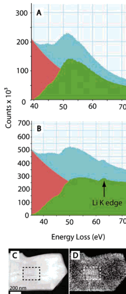
Figure 2. (A–B) EELS spectra of NRs with background extrapolated using log polynomial law fitting. The pink is the background, the blue is the total signal, and the green is extracted NR signal. (A) Spectrum taken from pristine \text{V}_2\text{O}_5 NR with V M45-edge onset seen at \sim 37 eV. (B) Spectrum taken from \text{Li}_x\text{V}_2\text{O}_5 NR with the V M45-edge onset seen at \sim 37 eV and Li K resonance at \sim 62 eV. The Li K resonance is not observed in the pristine NR spectrum. (C) STEM image of \text{Li}_x\text{V}_2\text{O}_5 NR with a dashed box indicating a crack in the structure. (D) Corresponding EELS spectrum image (same scale as Figure 2C) spatially mapping the signal from the Li K edge resonance. The brighter spots correspond to the higher Li signal, notably around the edges of the NR and the crack inside the dashed box.
